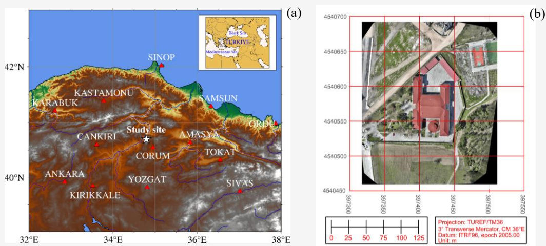
Figure 1: Location and spatial characteristics of the test building: (a) regional location map, where the white star represents the position of the test site, and (b) ortho-mosaic view of the test site and selected façades of the building (blue). Projected coordinates in (b) are presented in the TUREF/TM36 coordinate reference system (3° Transverse Mercator; central meridian 36°E; units: m)
