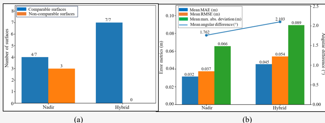
Figure 7: Overall surface representation performance of the nadir and hybrid photogrammetric models. Panel (a) shows the number of comparable and non-comparable reference surfaces, while panel (b) summarizes the mean surface error metrics and the mean angular difference between reference and photogrammetric surfaces
